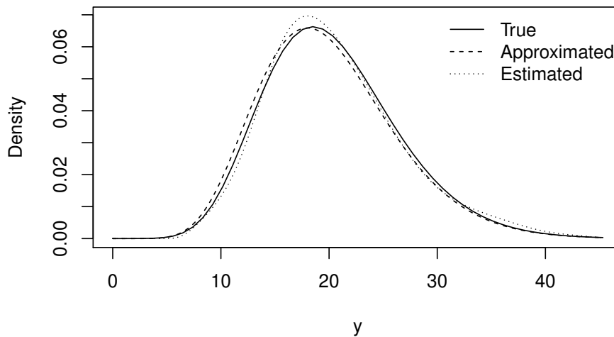
Figure 16: \chi_{20}^2 Data. Density of a \chi_{20}^2 (true), an approximating unconditional transformation model and the density fitted to a sample from the approximating model.
